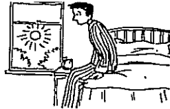
2 He .....
